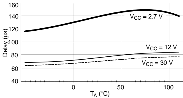
Figure 20. Shutdown Delay vs. T_A
