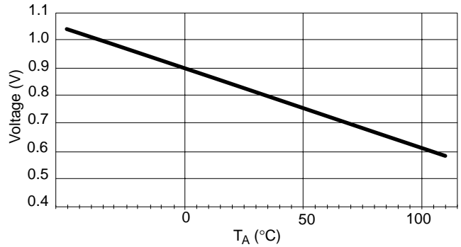
Figure 19. Shutdown Threshold vs. T_A
